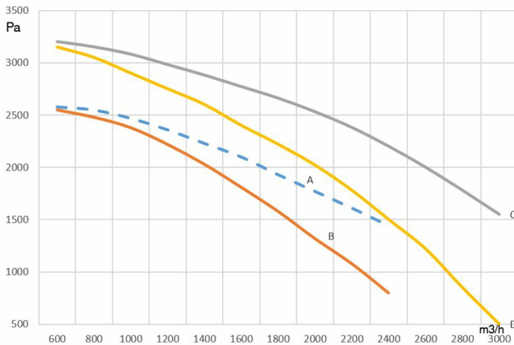
A = Fan total pressure (1,5 kW) B = Fan static pressure (1,5 kW) C = Fan total pressure (2,2 kW) D = Fan static pressure (2,2 kW)
